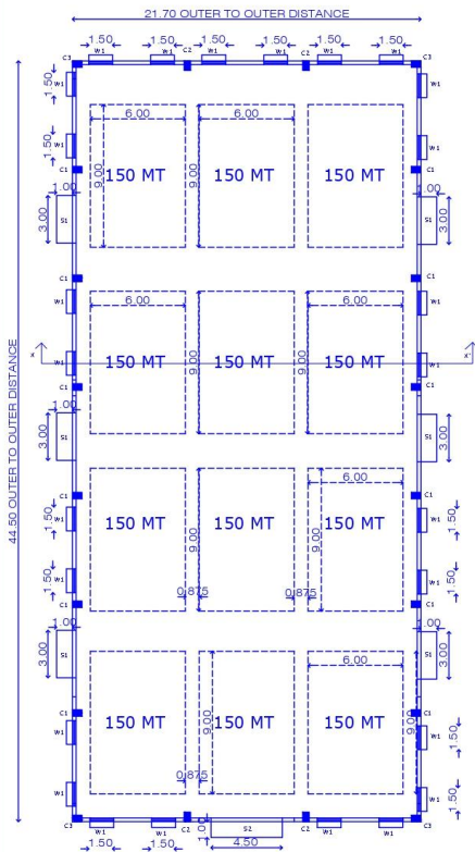
PLAN FOR 1800 MT.WH.
