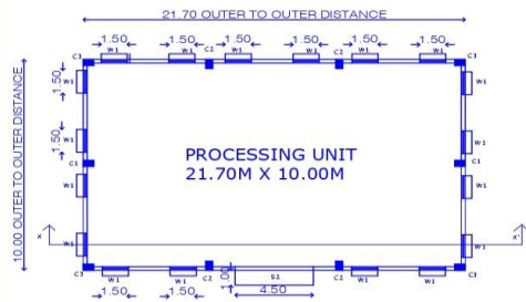
PLAN FOR PROCESSING UNIT
